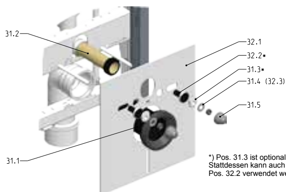
Detail B
