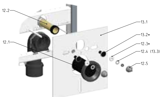
Detail A 1:5
